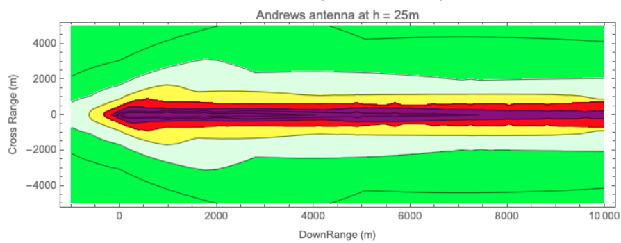
Figure 24 Radiation Pattern with Antenna at 25m
