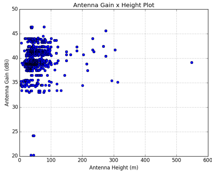
Figure 16 Microwave Antenna Gain x Height Scatter Diagram
