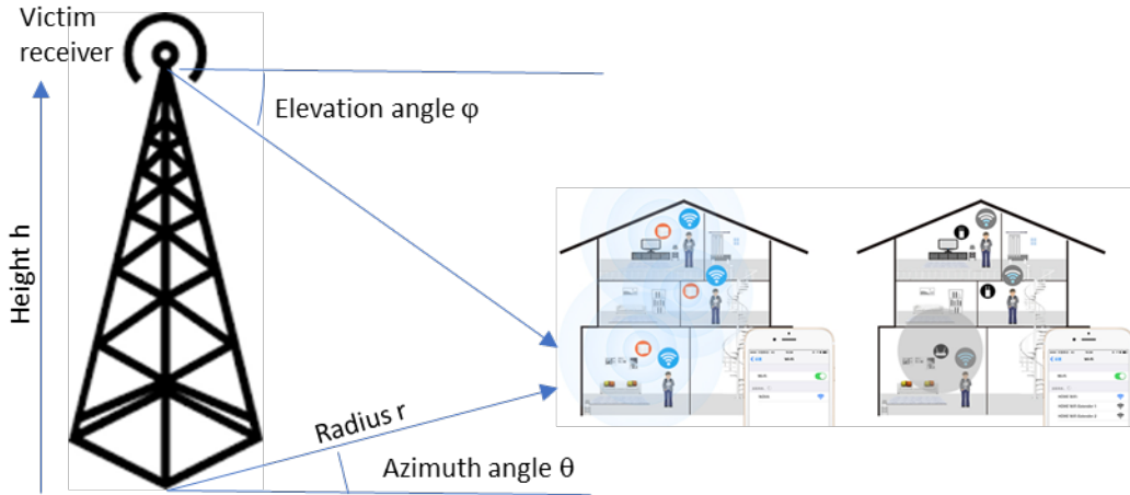
Figure 11 Radius, Azimuth, Elevation Geometry
