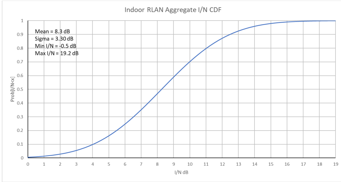
Figure 17 Indoor RLAN I/N Probability Distribution
