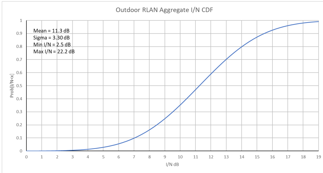
Figure 7 Outdoor RLAN I/N Distribution
