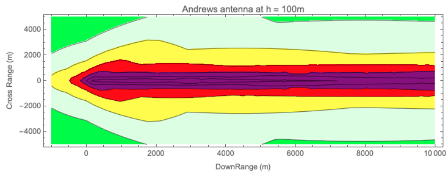
Figure 23 Radiation Pattern with Antenna at 100m
