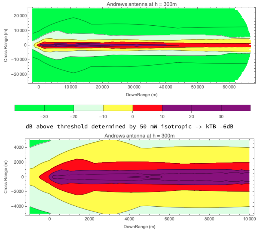
Figure 25 Radiation Pattern with Antenna at 300m
