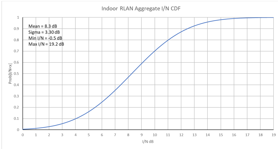
Figure 6 Indoor I/N Distribution
