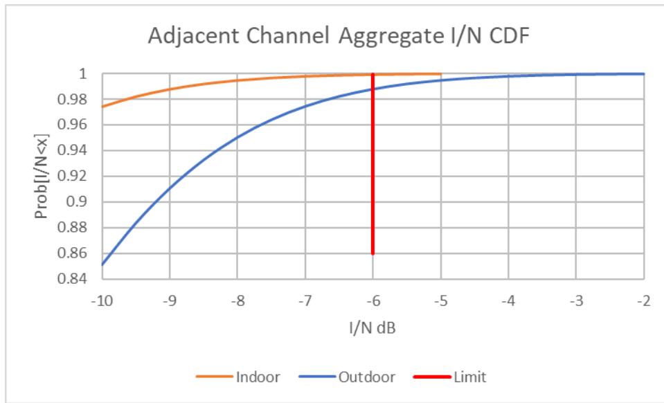
Figure 8 Adjacent Channel I/N Distributions
