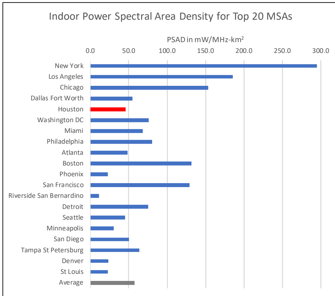
Figure 27 Indoor PSADs for Top 20 MSAs
