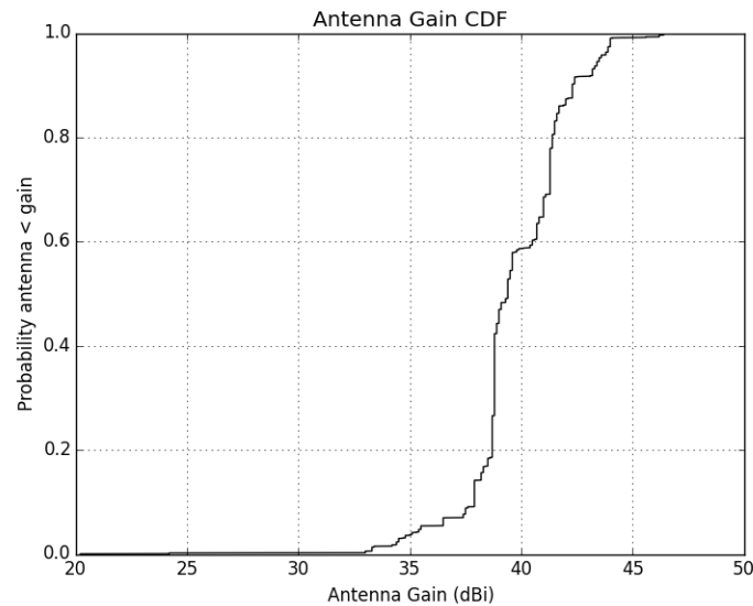
Figure 15 Microwave Antenna Gain Distribution
