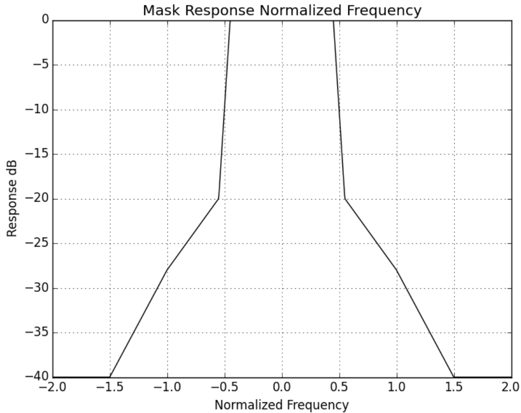
Figure 18 RLAN Adjacent Channel Emission Mask
