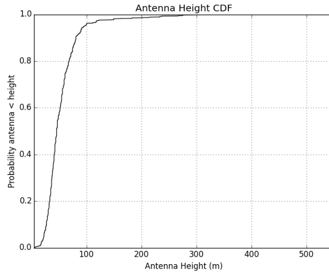
Figure 14 Microwave Antenna Height Distribution
