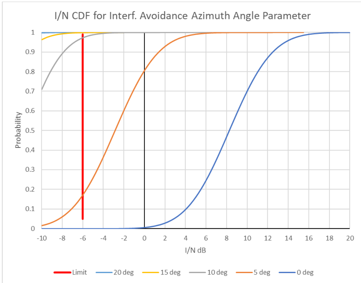
Figure 20 I/N with IAAA Parameter
