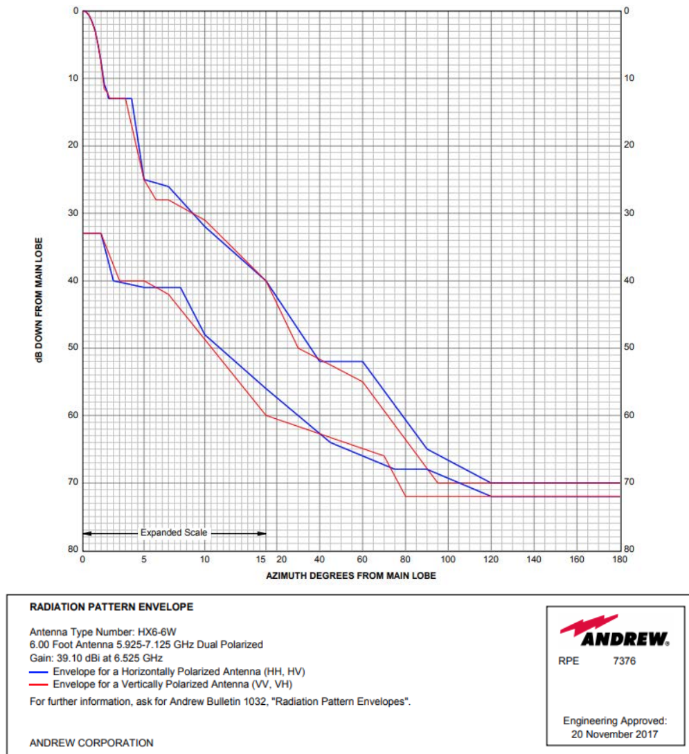
Figure 5 Typical Point-to-Point Antenna Gain Function
