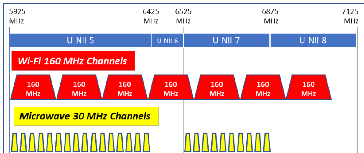
Figure 1 Radio Channels in 6 GHz
