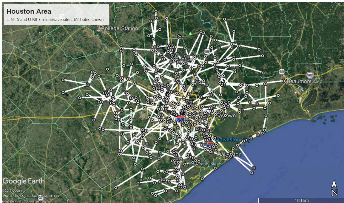
Figure 13 Houston Microwave Link Paths
