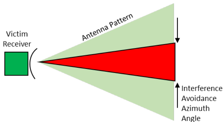
Figure 19 Interference Avoidance Azimuth Angle
