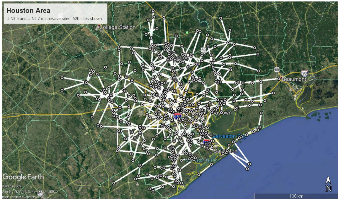
Figure 4 Houston Microwave Link Paths
